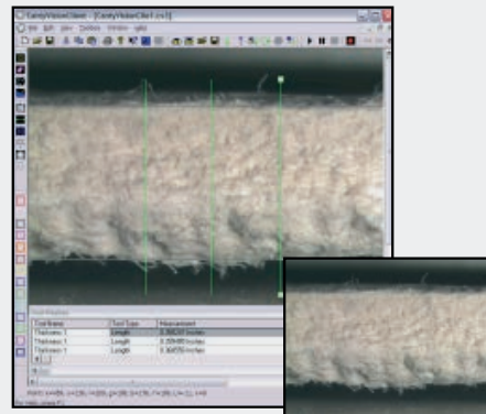
Analyzed Image by CantyVision™ with STANDARD EDGE METHOD Thickness Measurement
