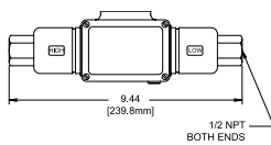
Models S147B-S157B
