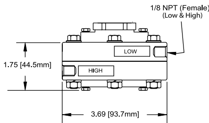
Models 544-547
