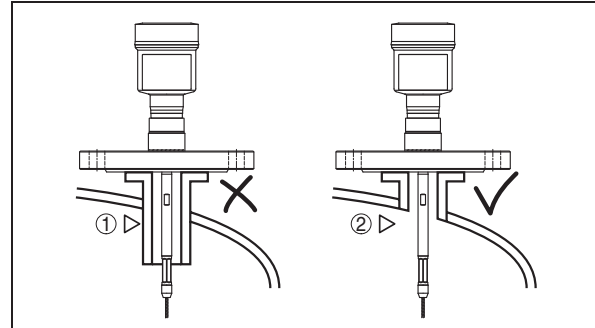
Fig. 10: Socket must be installed flush
