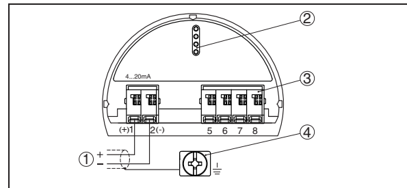
Fig. 18: Electronics and connection compartment, single chamber housing
