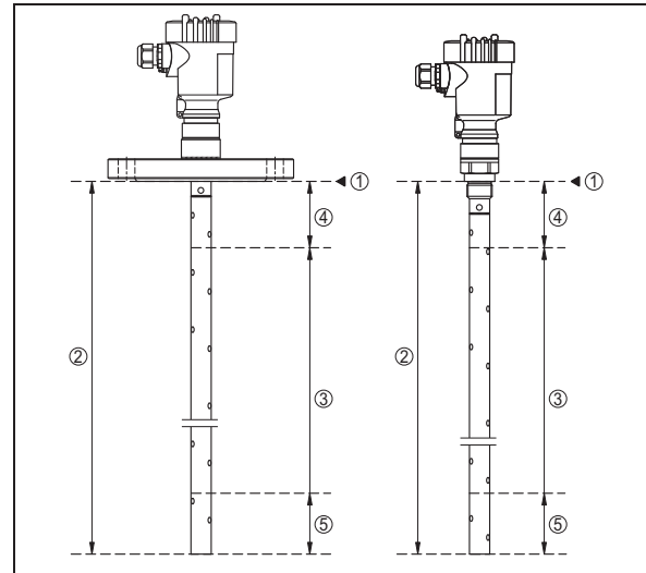
Fig. 3: Measuring ranges of VEGAFLEX - coax version
