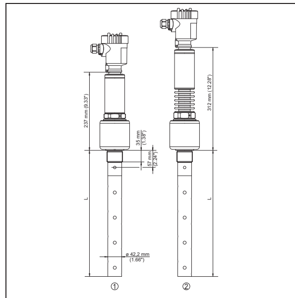
Fig. 42: VEGAFLEX 86, coax version with threaded fitting
