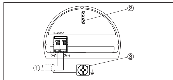
Fig. 19: Connection compartment, double chamber housing
