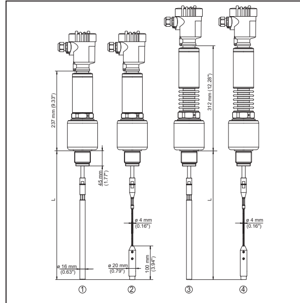
Fig. 40: VEGAFLEX 86, cable, rod version with threaded fitting
