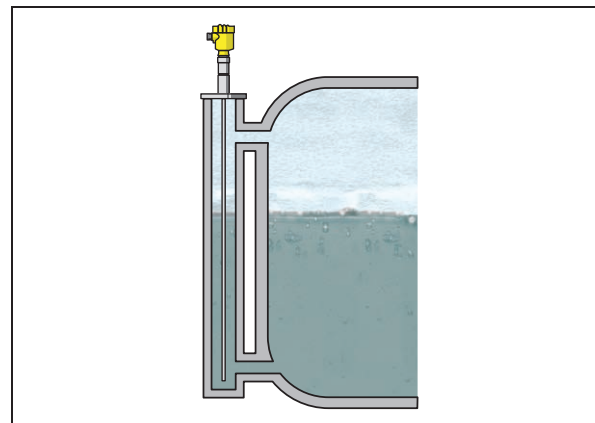
Fig. 17: Level measurement in a bypass tube
