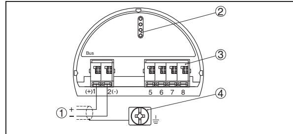
Fig. 26: Connection compartment, double chamber housing
