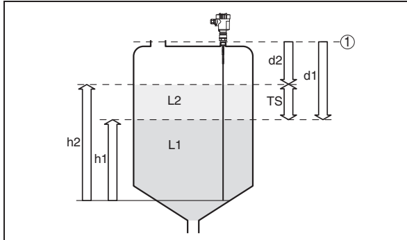
Fig. 8: Interface measurement
