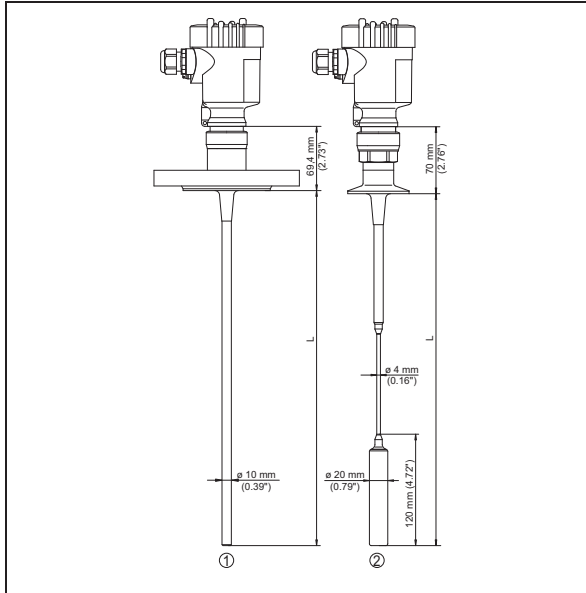
Fig. 36: VEGAFLEX 83, PFA coated version
