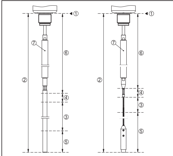
Fig. 12: Measuring ranges - VEGAFLEX with steam compensation
