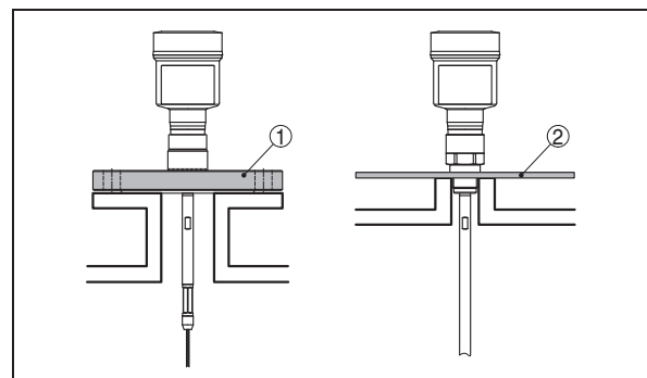
Fig. 11: Installation in non-metallic vessel
