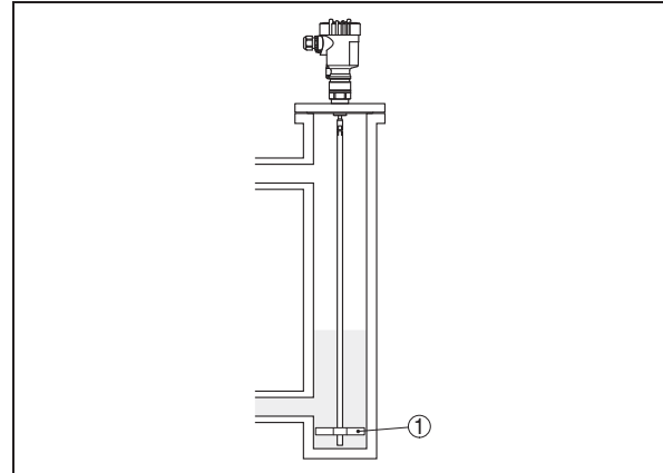
Fig. 7: Position of the spacer
