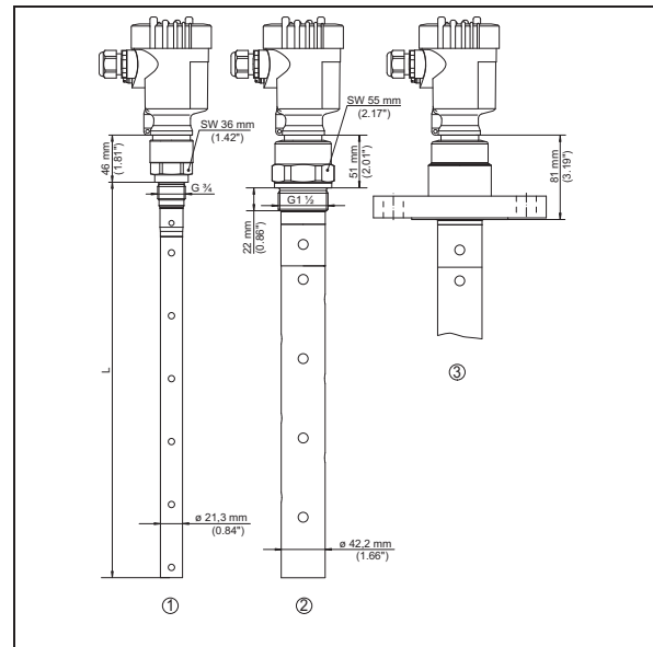
Fig. 34: VEGAFLEX 81, coax version
