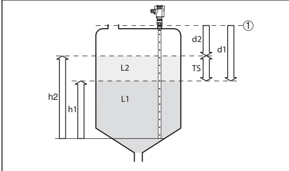
Fig. 5: Interface measurement
