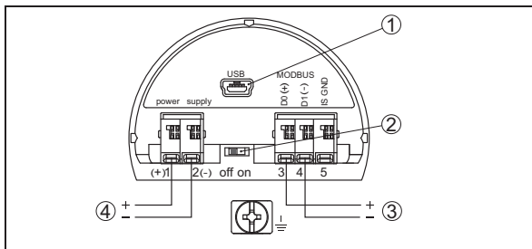
Fig. 28: Connection compartment
