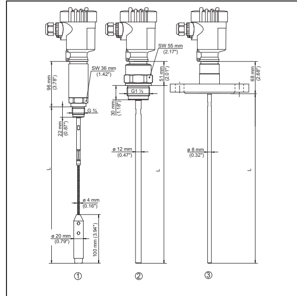
Fig. 32: VEGAFLEX 81, cable and rod version
