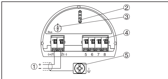
Fig. 25: Electronics and connection compartment, single chamber housing
