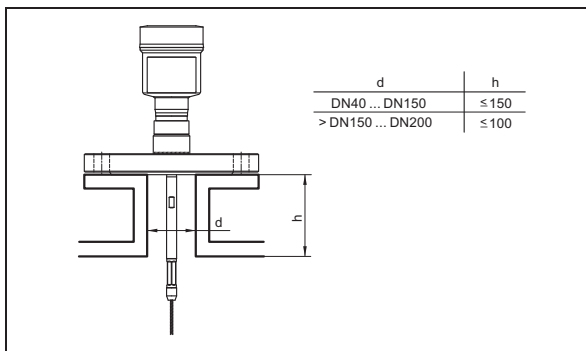
Fig. 9: Mounting socket
