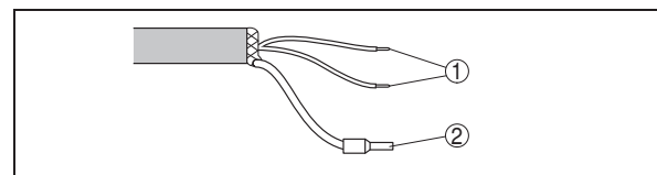
Fig. 20: Wire assignment fix-connected connection cable
