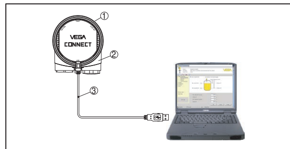
Fig. 31: Connection via VEGACONNECT and USB
