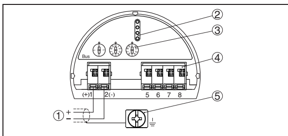
Fig. 22: Electronics and connection compartment, single chamber housing
