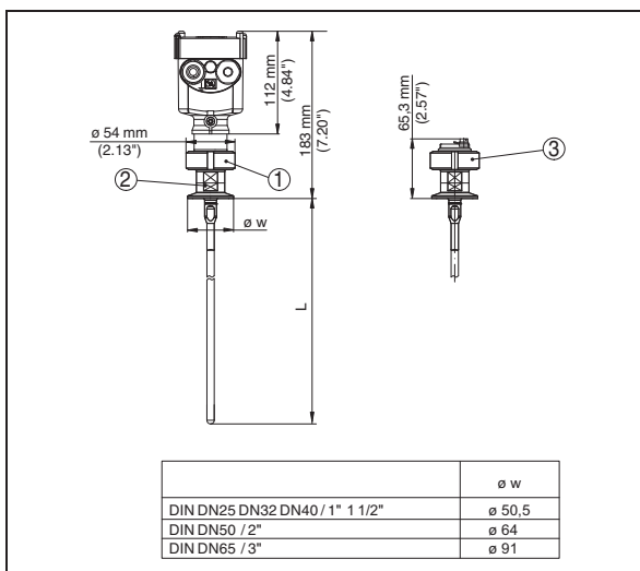
Fig. 14: Autoclaved version
