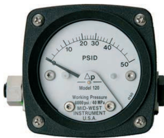
Model 120 0-50 PSID 2-1/2" Dial
