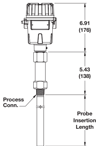
Model 7XP Probe Threaded Connection
