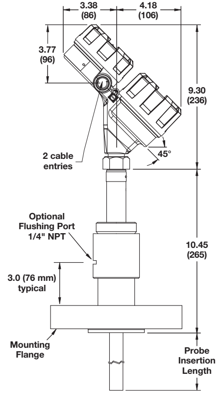
Model 7yD with flanged connection
