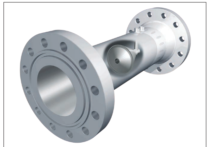
Figure 3: V-Cone Flowmeter Cutaway
