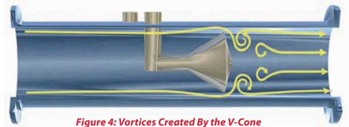
Figure 4: Vortices Created By the V-Cone
