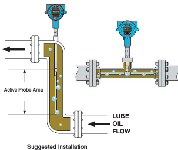
Lube Oil Monitor Mounted in vertical section of pipe. Monitor can also be mounted directly in lube oil reservoir.
