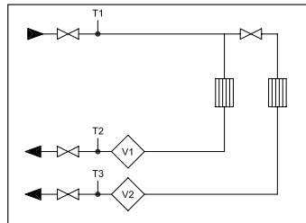
Example 3: 2 heat circuits with joint flow
