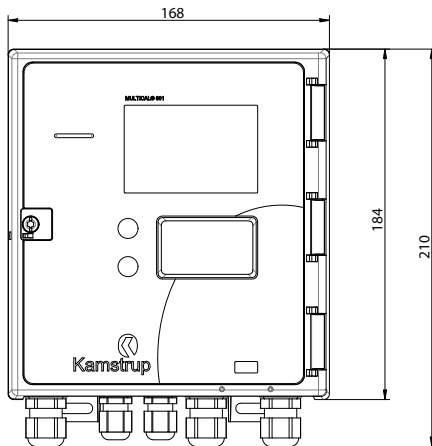
Front dimensions of MULTICAL® 801
