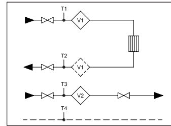
Example 2: Closed thermal system with 2 flow sensors
