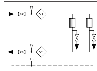
Example 4: Open system with 2 flow sensors
