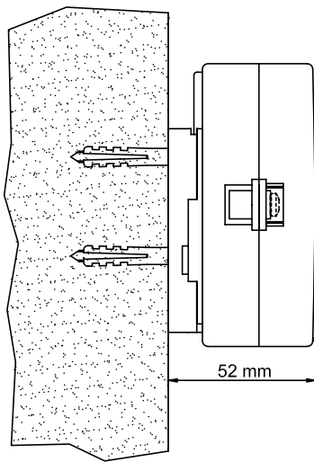
Wall-mounted MULTICAL® 602 seen from the side
