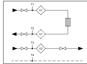
Example 2: 2 string system with 2 flow sensors
