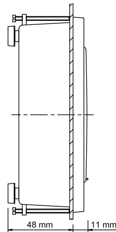
Panel-mounted MULTICAL® 602 seen from the side
