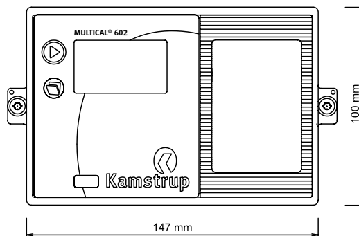
Front dimensions of MULTICAL® 602
