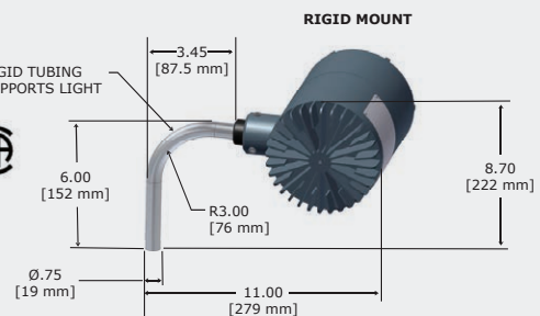
Typical 12" Direct Mount Light Bundle Models
