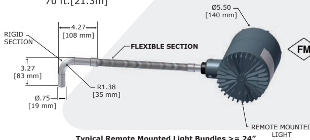
Typical Remote Mounted Light Bundles >= 24"
