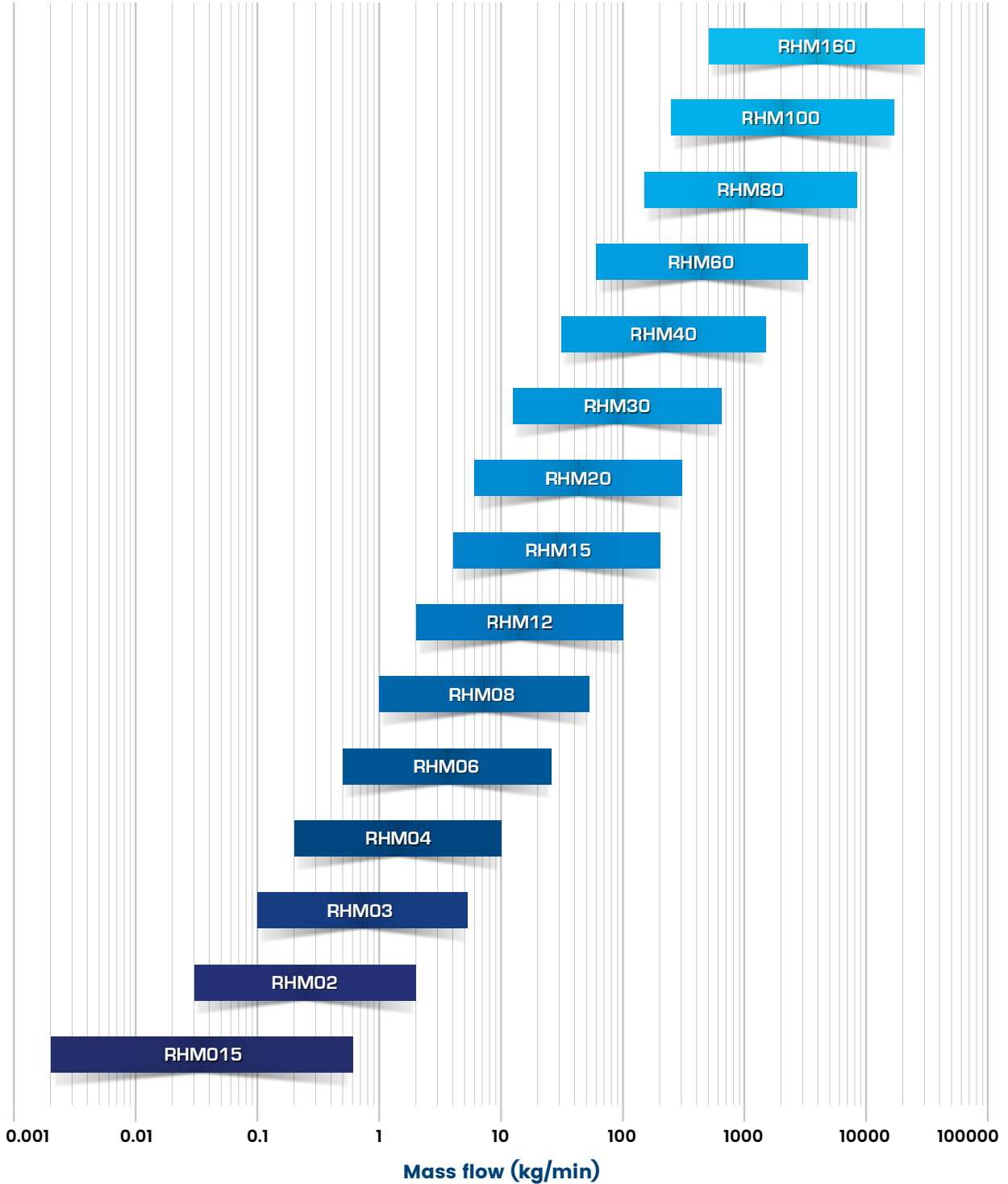
Flow rate chart depicts flow ranges for liquid applications at typical/common process pressure ratings. Flow ranges for meters with higher pressure ratings may vary. Gas flow ranges will depend upon pressure.
