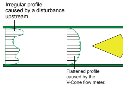
Flattened Velocity Profile Figure 3
