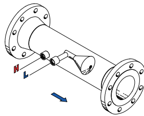
Precision Tube V-Cone Flow Meter Figure 7
