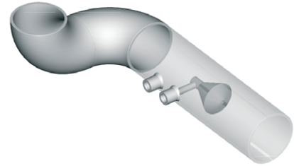
Double Elbow and V-Cone Flow Meter Figure 5
