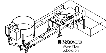
Calibration Facility 40k Gravimetric Figure 9
