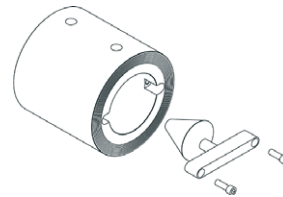
Wafer-Cone Flow Meter Figure 8
