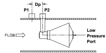
High and Low Ports Figure 1
